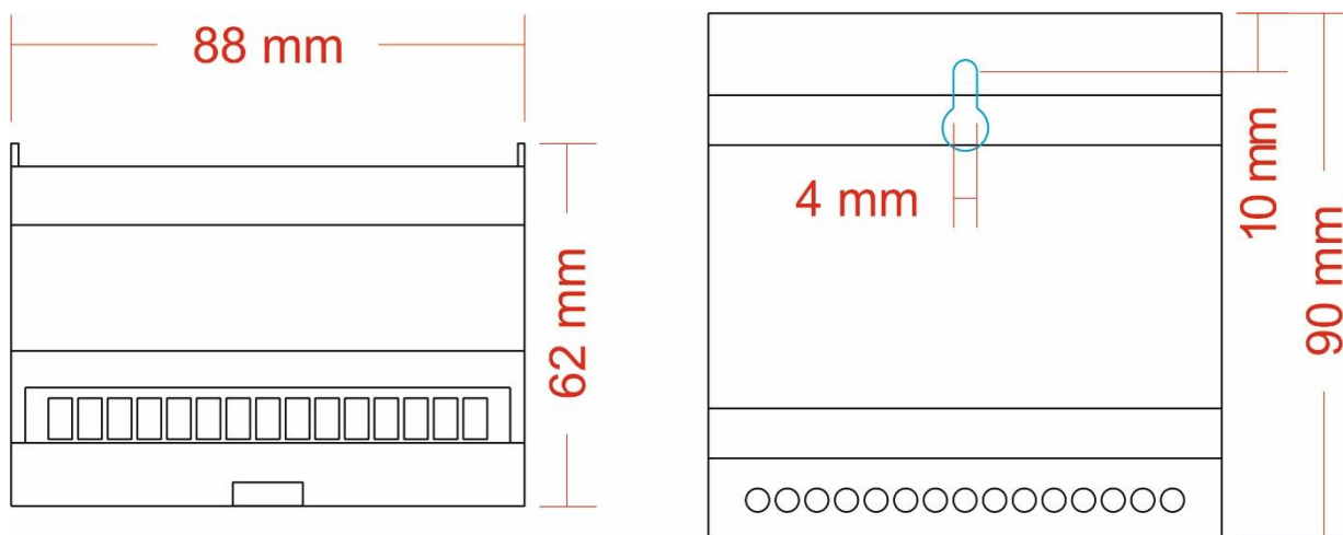
Mounting Drawing
